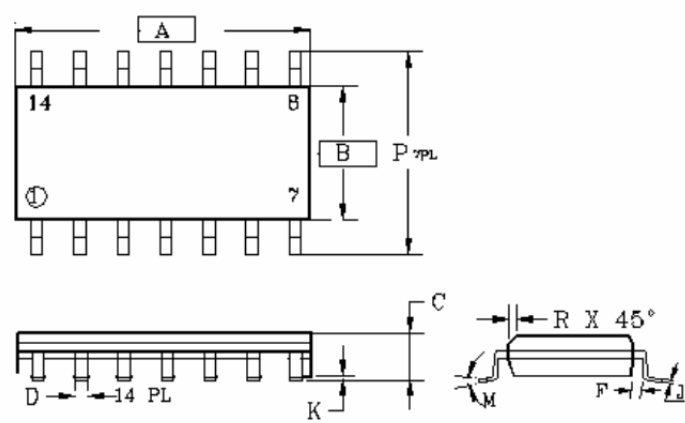
SOP-14
