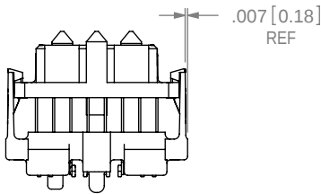
-07.0 LEAD STYLE (SEAM-XX-07.0-X-08-A-X SHOWN)
