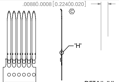
DETAIL 'H' SCALE 16:1
