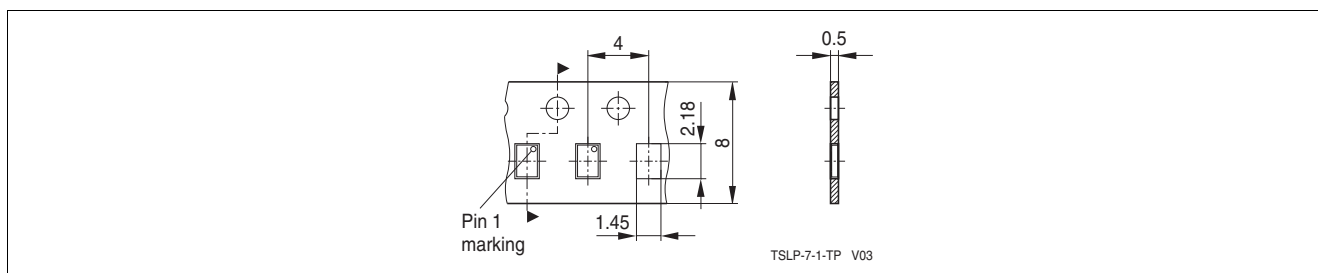
Figure 9 Tape & Reel Dimensions
