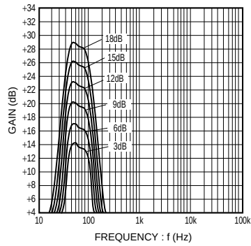
Fig.8 Biamp characteristics (Input common-mode)
