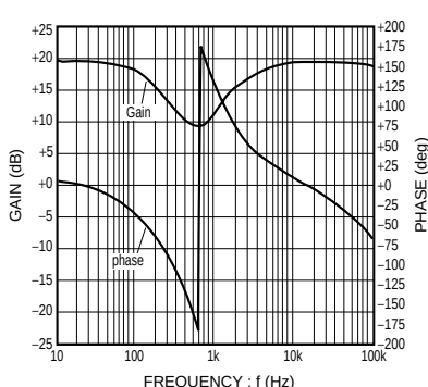
Fig.6 Surround characteristics
