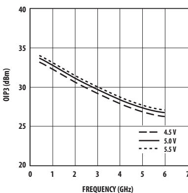
Figure 7. Output Third Order Intercept Point vs. Frequency and Voltage [2] .
