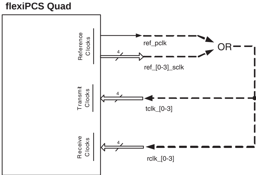
Figure 6-12. Synchronous input clocks to flexiPCS quad set to Fibre Channel Mode
