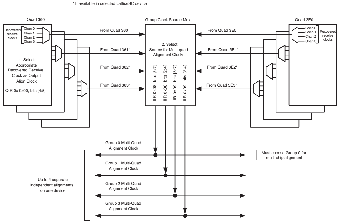
Figure 11-13. Multi-quad Alignment Group Clock Source Setup
