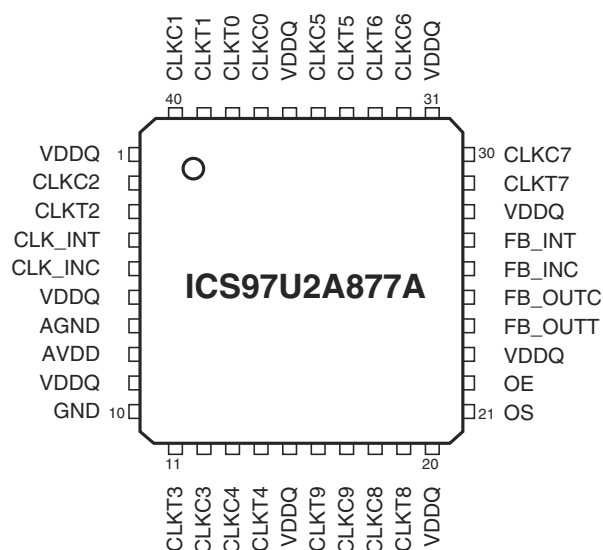
40-Pin MLF
