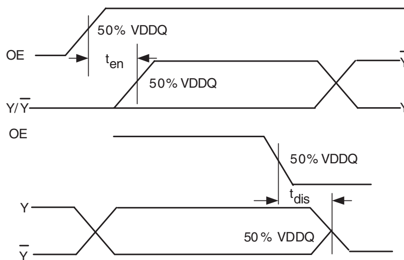
Figure 10. Time delay between OE and Clock Output (Y, \bar{Y} )
