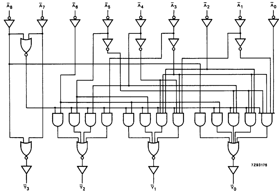
Fig.5 Logic diagram.
