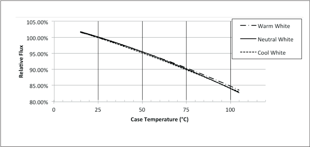
Figure 4: Typical DC Flux vs. Case Temperature
