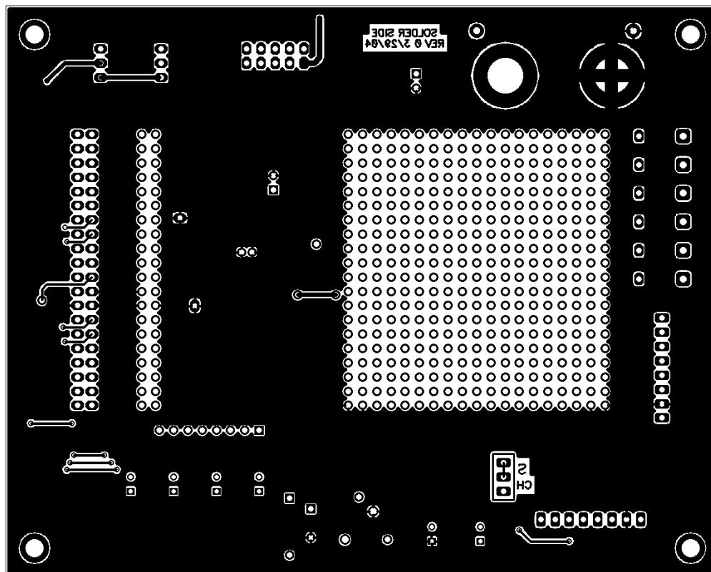
Figure 6. Bottom-side Foil
