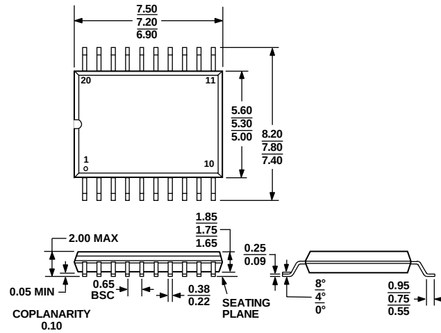
Figure 34. 20-Lead Shrink Small Outline Package [SSOP] (RS-20)
