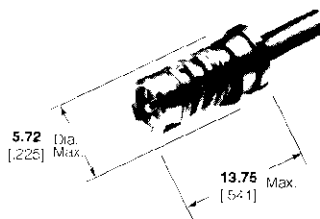
RG-405 Semi-Rigid/2.18 [.086] Cable Part No. 413249-1
