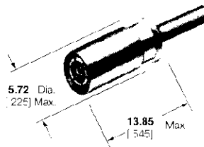
RG-405 Semi-Rigid/2.18 [.086] Cable Part No. 413242-1
