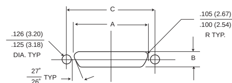
Plug and Rectacle Dimensions
