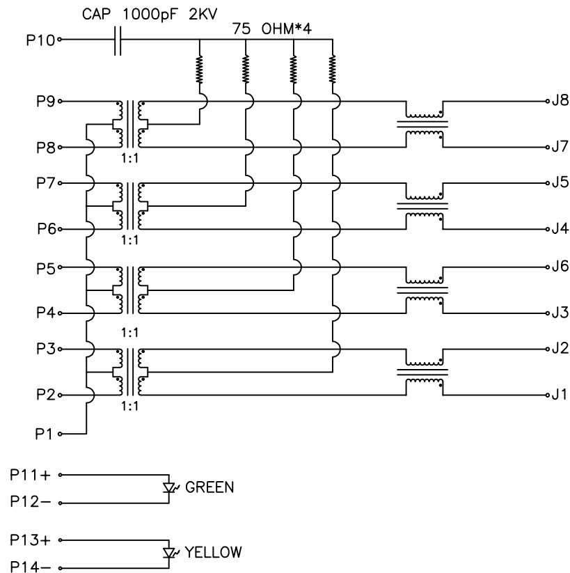
SCHEMATIC
