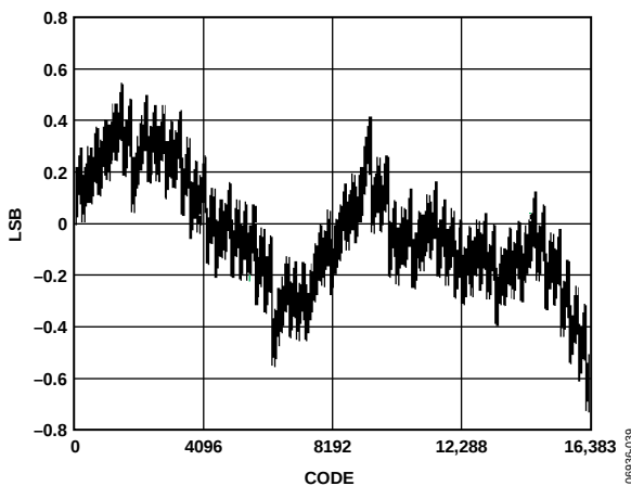
Figure 39. AD9781 INL, FS = 20\text{ mA}
