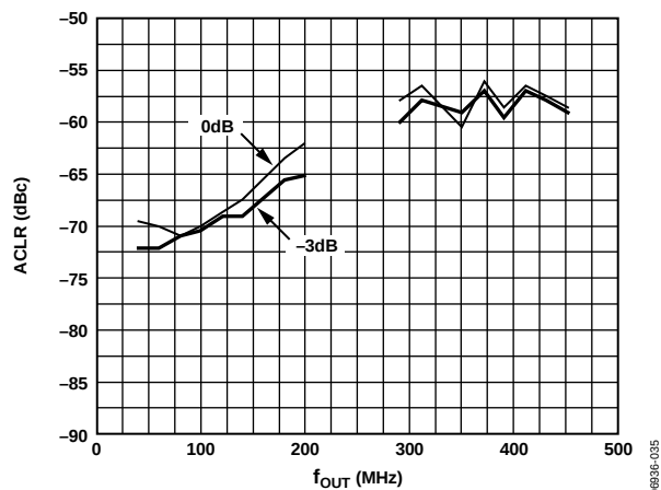
Figure 35. AD9783 ACLR for First Adjacent Channel Four-Carrier W-CDMA Over Digital Input Level Baseband and Mix Modes, at 491.52 MSPS, FS = 20\text{ mA}
