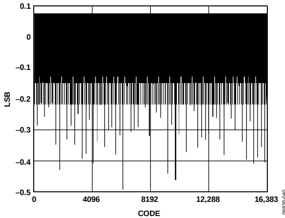
Figure 40. AD9781 DNL, FS = 20\text{ mA}
