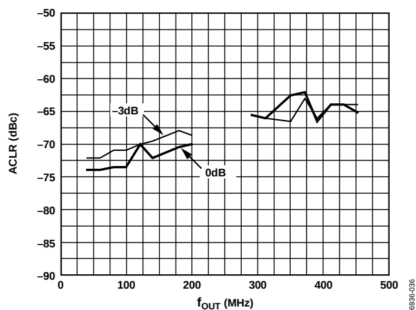
Figure 36. AD9783 ACLR for Second Adjacent Channel Four-Carrier W-CDMA Over Digital Input Level Baseband and Mix Modes, at 491.52 MSPS, FS = 20\text{ mA}
