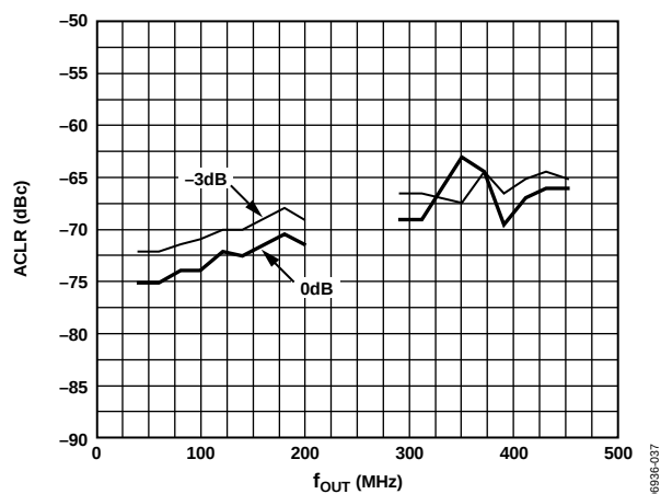
Figure 37. AD9783 ACLR for Third Adjacent Channel Four-Carrier W-CDMA Over Digital Input Level Baseband and Mix Modes, at 491.52 MSPS, FS = 20\text{ mA}
