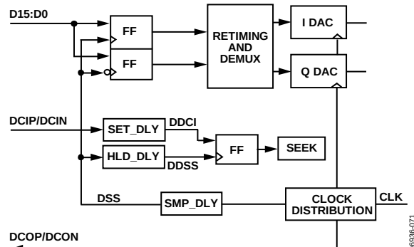
Figure 56. Digital Data Port Block Diagram
