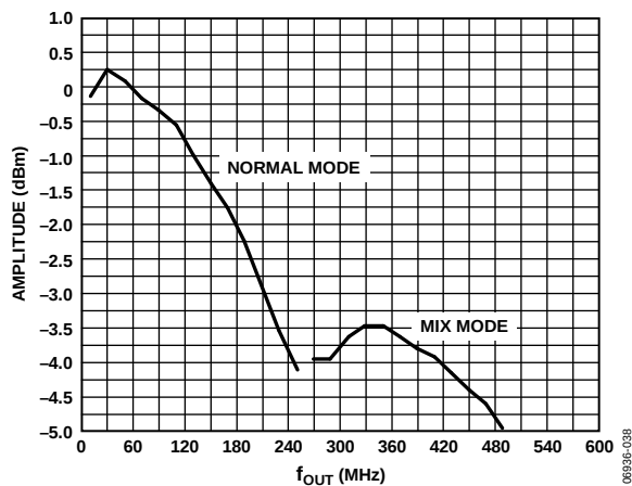
Figure 38. Nominal Power in the Fundamental, FS = 20\text{ mA} , at 500 MSPS, FS = 20\text{ mA}
