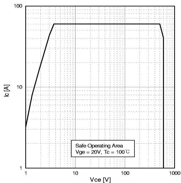
Fig.11 Turn-off SOA
