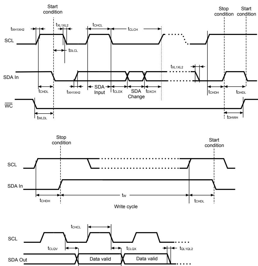
Figure 14. AC waveforms
