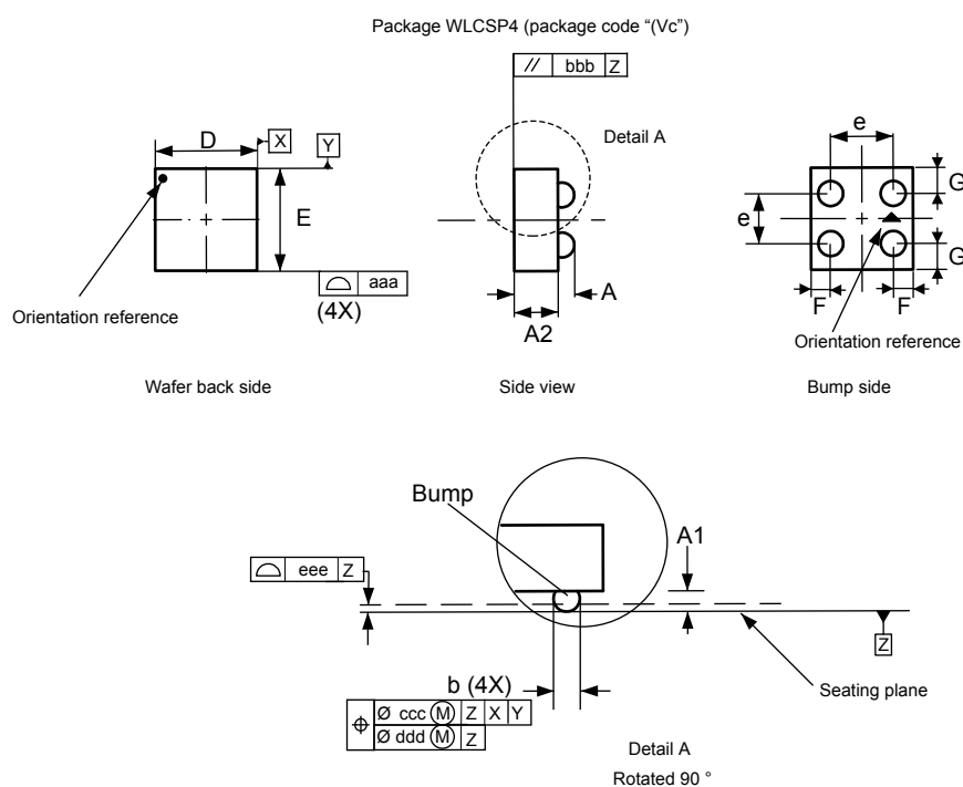
Figure 15. WLCSP4 - Outline
