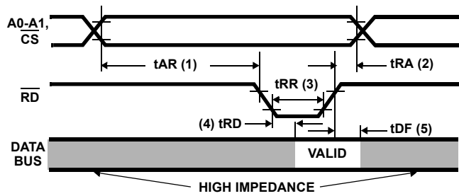
FIGURE 31. READ TIMING
