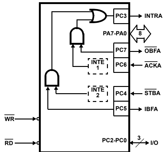
FIGURE 12. MODE 2
