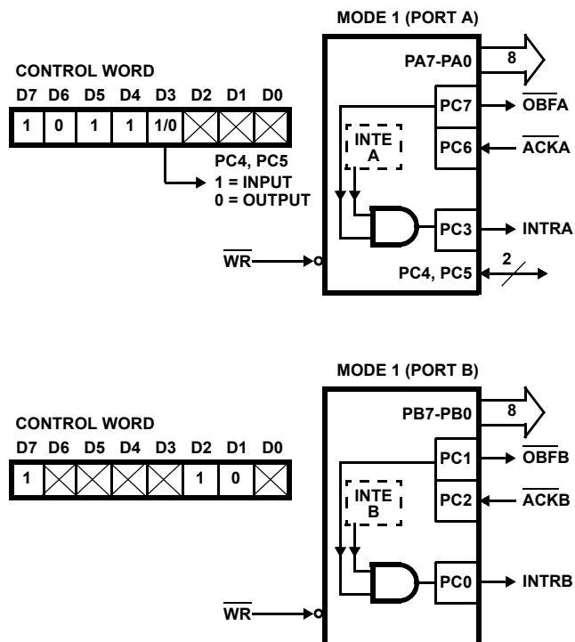
FIGURE 8. MODE 1 OUTPUT
