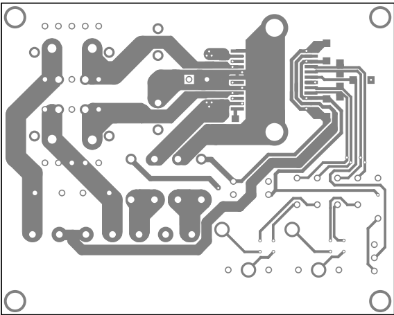
Top copper
