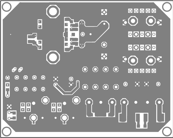
Bottom copper
