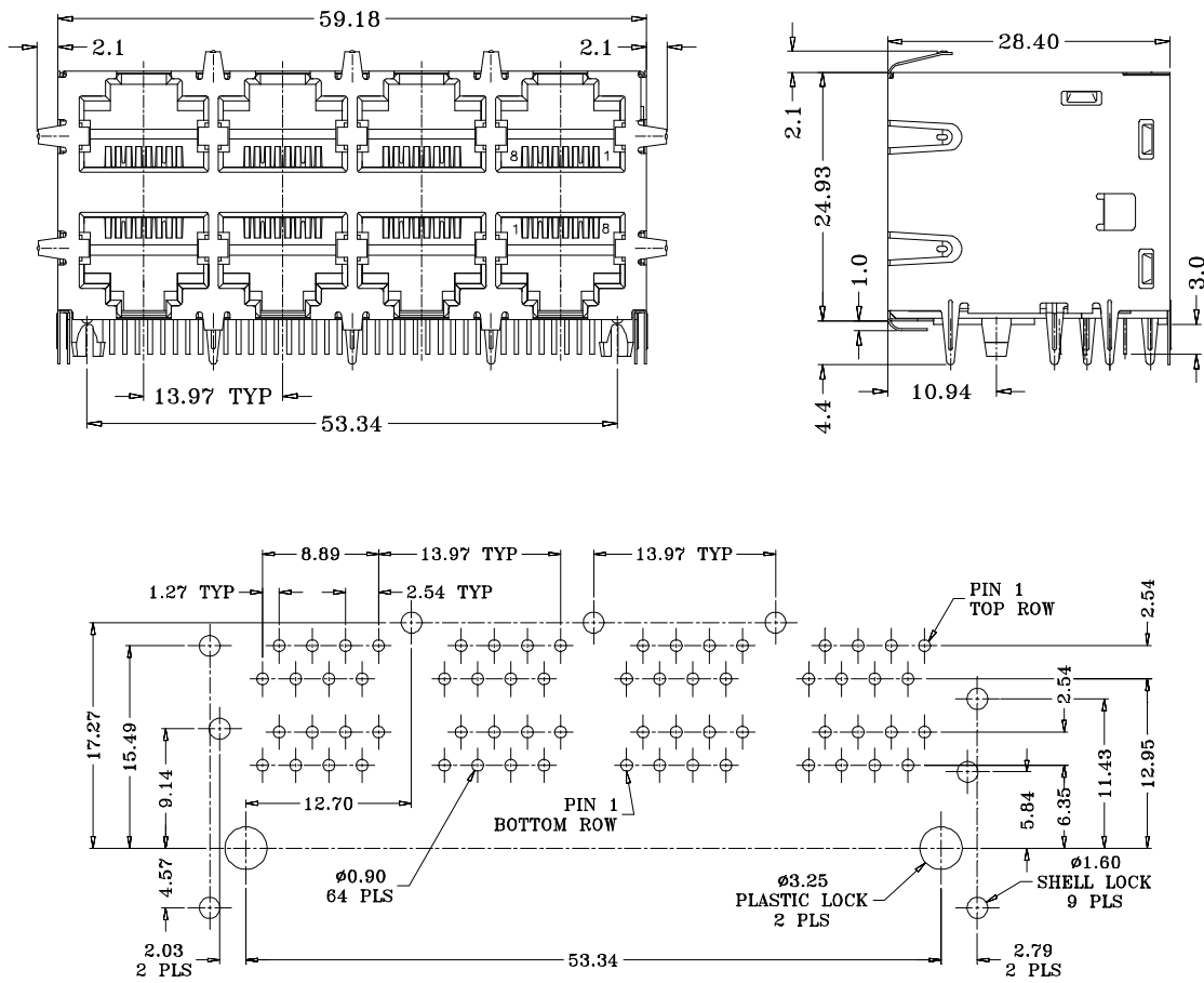
RECOMMENDED PCB LAYOUT (COMPONENTS SIDE)
