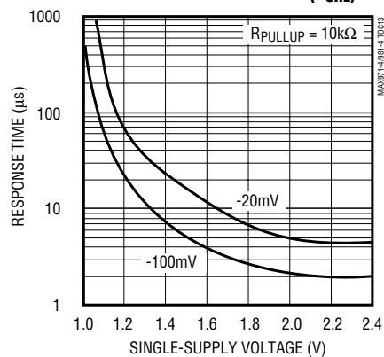
RESPONSE TIME AT LOW SUPPLY VOLTAGES (V OHL )
