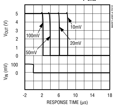
RESPONSE TIME FOR VARIOUS INPUT OVERDRIVES (V OHL )
