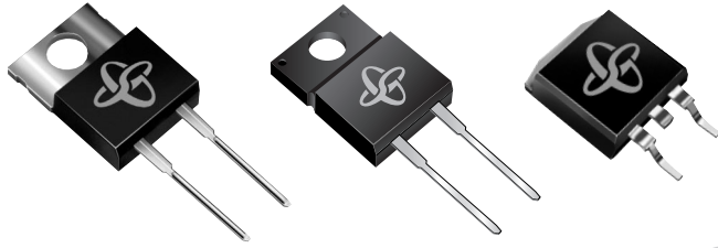
TO-220AC (MBR1090, MBR10100)
