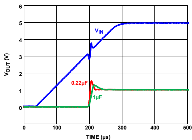
FIGURE 12. TURN-ON TIME
