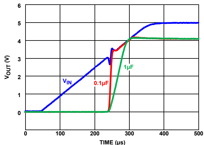
FIGURE 131. TURN-ON TIME
