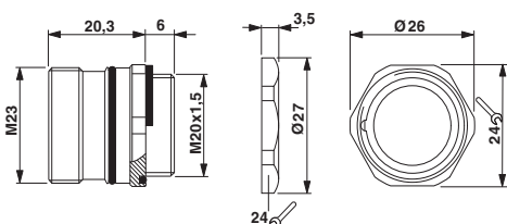
RC-00000006100 O-Ring axial
