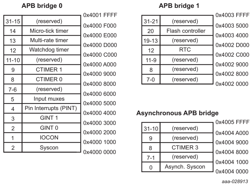
Fig 6. LPC51U68 APB Memory map
