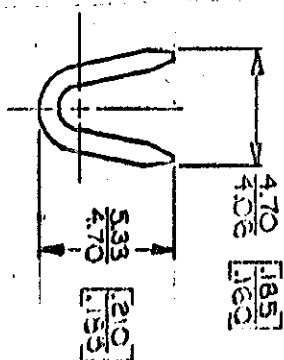
SECT. A-A
