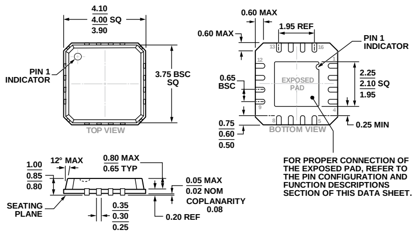
Figure 33. 16-Lead Lead Frame Chip Scale Package [LFCSP_VQ] 4 mm x 4 mm Body, Very Thin Quad (CP-16-4)
