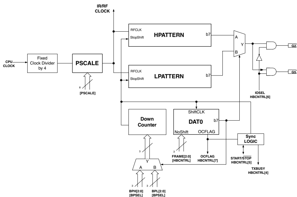
Figure 21: Hardware Bit-Coder (HBC) Block Diagram
