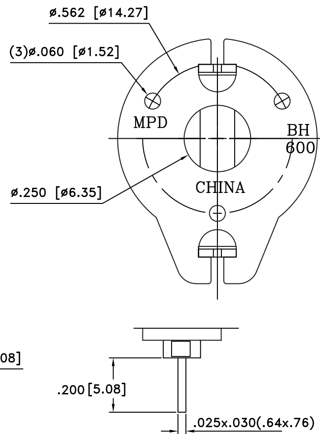
Square Contact Detail
