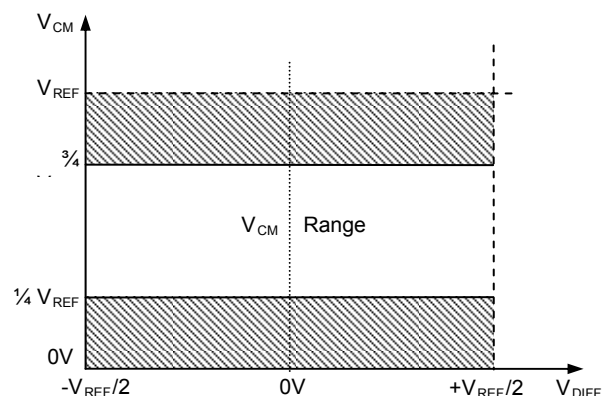
Figure 7: Input voltage range for bipolar mode
