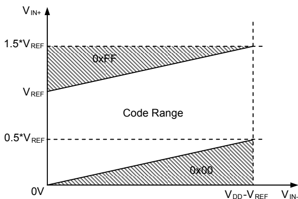
Figure 6: Input voltage range in unipolar mode
