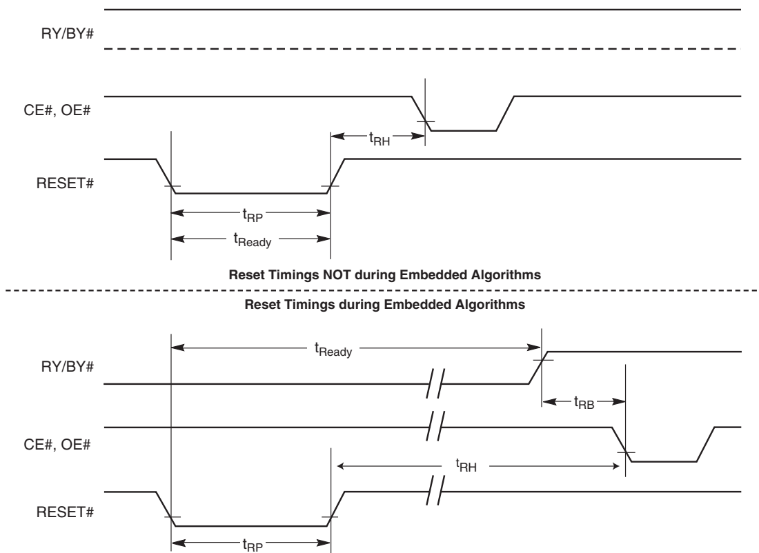
Figure 15.2 RESET# Timings
