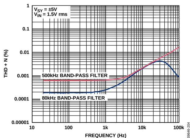
Figure 44. THD + N vs. Frequency, V_{SY} = \pm 5\text{ V}
