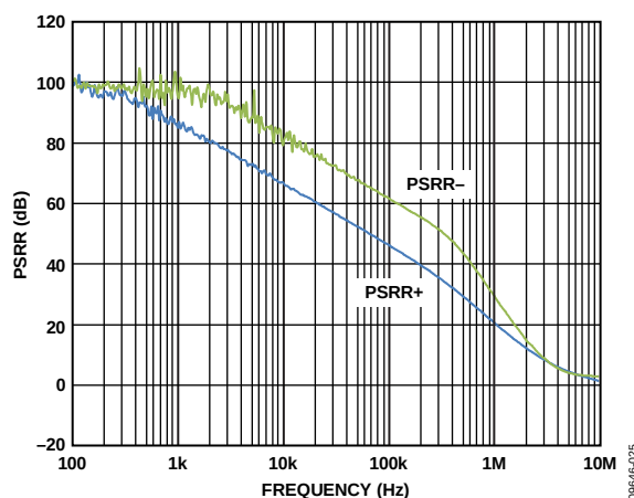
Figure 32. PSRR vs. Frequency, V_{SV} = \pm 15\text{ V}
