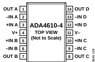
Figure 7. ADA4610-4 Pin Configuration, 14-Lead SOIC (R Suffix)
