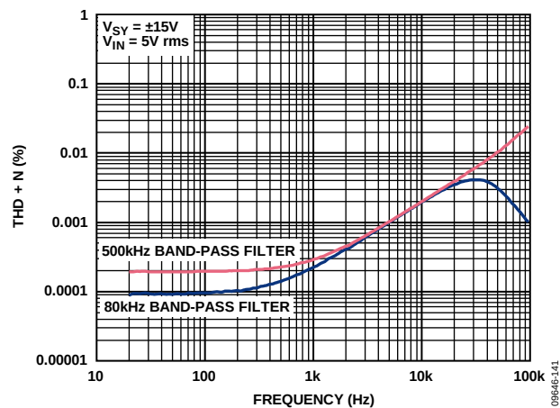
Figure 47. THD + N vs. Frequency, V_{SY} = \pm 15\text{ V}
