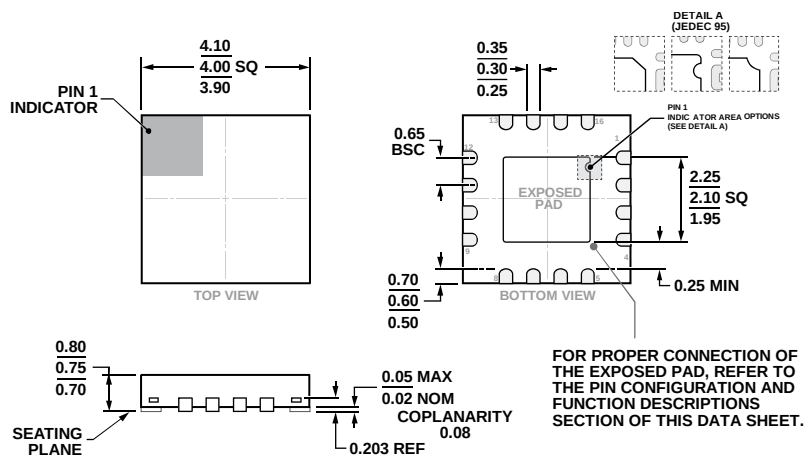
Figure 69. 16-Lead Lead Frame Chip Scale Package [LFCSP] 4 mm × 4 mm Body and 0.75 mm Package Height (CP-16-23)
