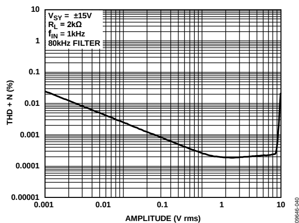
Figure 46. THD + N vs. Amplitude, V_{SY} = \pm 15\text{ V}
