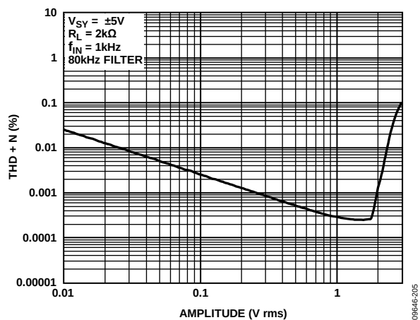
Figure 43. THD + N vs. Amplitude, V_{SY} = \pm 5\text{ V}
