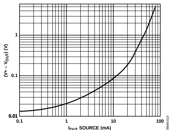
Figure 24. Dropout Voltage ( V^+ - V_{OUT} ) vs. I_{OUT} Source, V_{SY} = \pm 15 V
