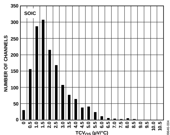
Figure 10. Input Offset Voltage Drift ( TCV_{OS} ) Distribution, V_{SY} = \pm 5\text{ V}
