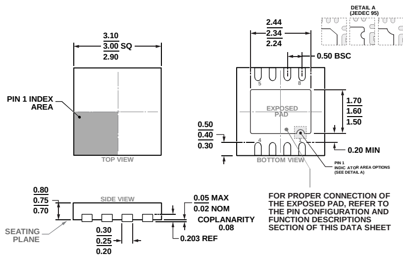
Figure 67. 8-Lead Lead Frame Chip Scale Package [LFCSF] 3 mm × 3 mm Body and 0.75 mm Package Height (CP-8-11)
