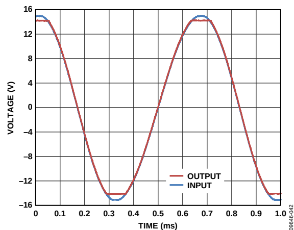
Figure 48. No Phase Reversal, V_{SY} = \pm 15\text{ V} , A_V = +1 , R_L = 2\text{ k}\Omega , C_L = 100\text{ pF}
