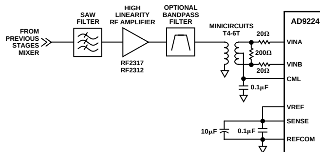
Figure 35. Example of AD9224 IF Sampling Circuit
