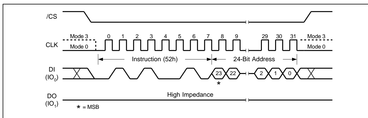
Figure 22a. 32KB Block Erase Instruction (SPI Mode)
