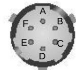
PPT-CE, PPTR Connector (pins—top view of PPT-CE, PPTR)
