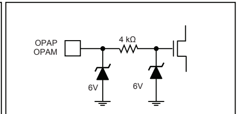
Figure 12h: Operational Amplifier Inputs
