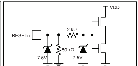
Figure 12e: RESETn Input
