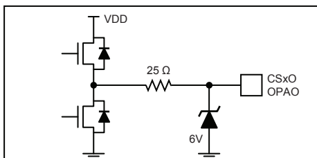
Figure 12i: Operational Amplifier and Current Sense Amplifier Outputs
