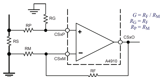
Figure 10: Basic current-sense amplifier configuration
