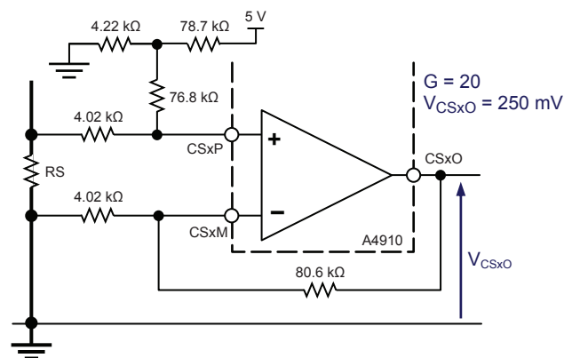
Figure 11: Typical current-sense amplifier configuration
