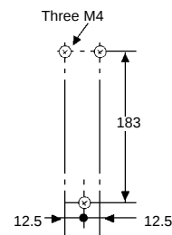
Mounting holes
