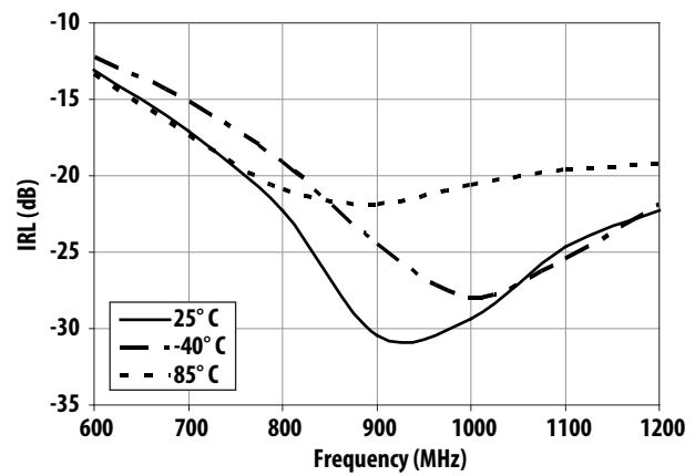
Figure 19. IRL vs Frequency and Temperature
