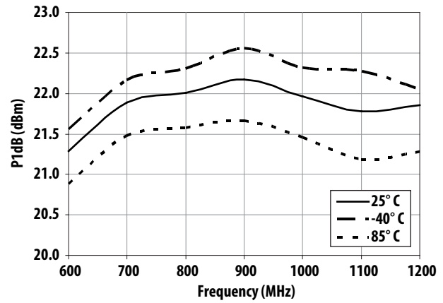
Figure 17. P1dB vs Frequency and Temperature
