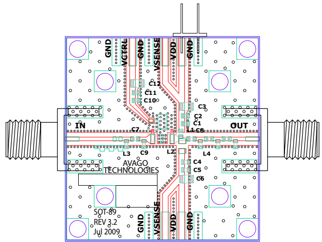
Figure 35. Demoboard
