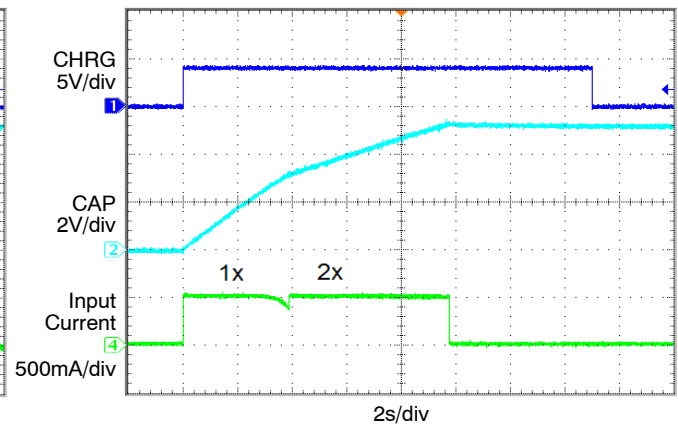
Figure 14. Charge Cycle, 500 mA Input Current
