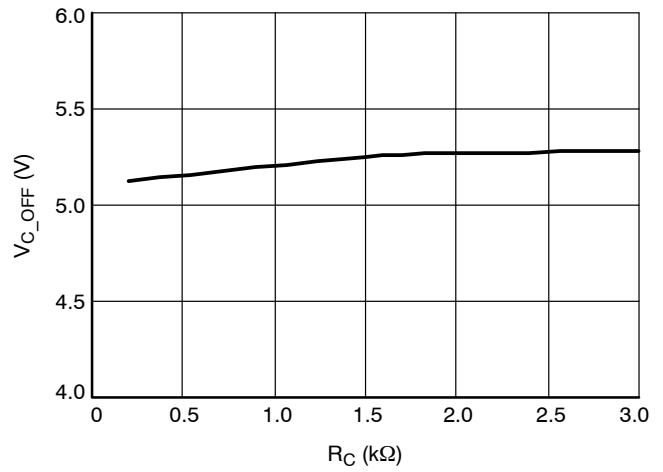
Figure 11. V CAP idle vs. R C
