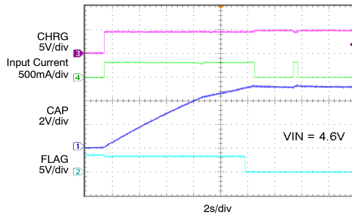
Figure 17. Charge Cycle with FLAG
