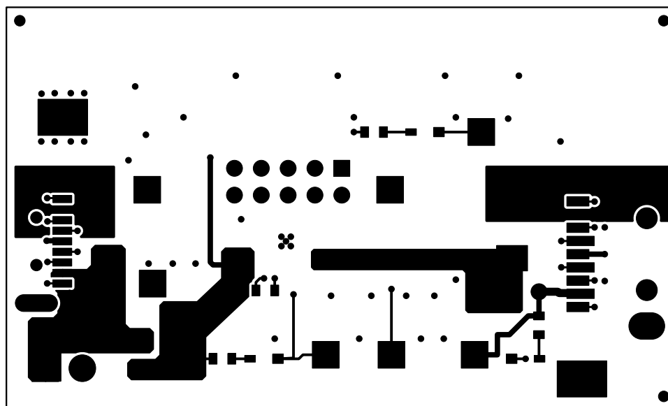
Figure 4. Top Side Routing
