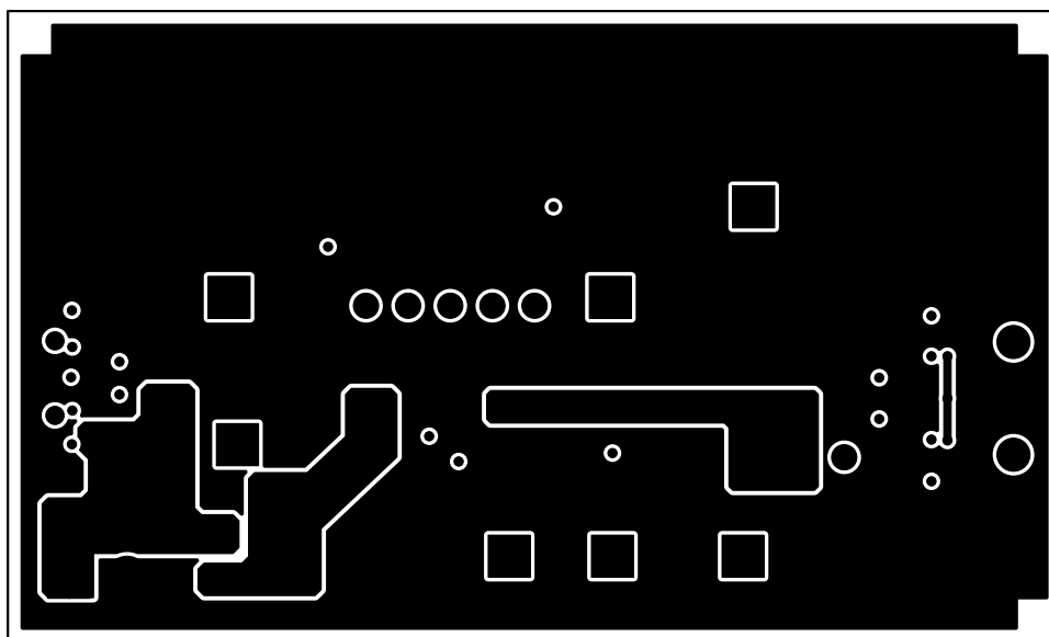
Figure 5. Layer Two Routing
