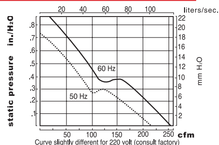
148VK Performance Curve
