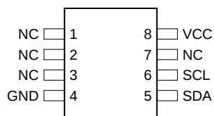
8-lead SOIC, PDIP or LAP
