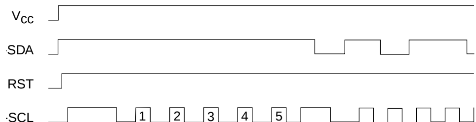
Figure 3. Synchronous 2-wire Protocol
