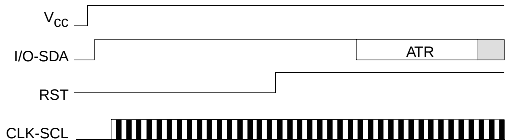
Figure 2. Asynchronous T = 0 Protocol
