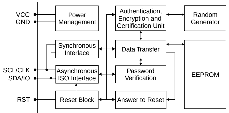
Figure 1. Block Diagram
