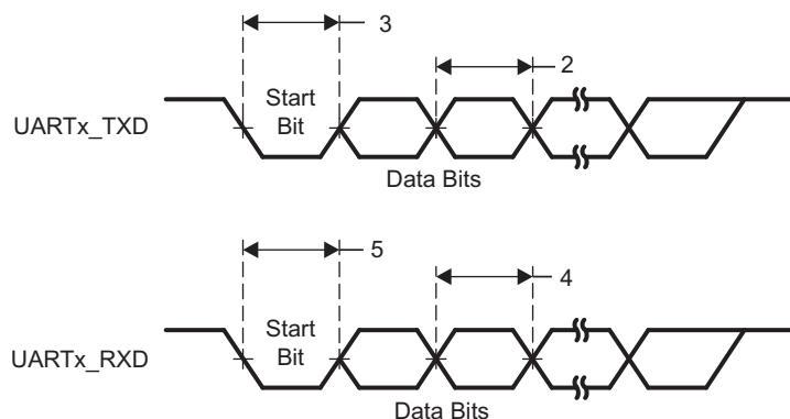
Figure 8-89. UART Timing
