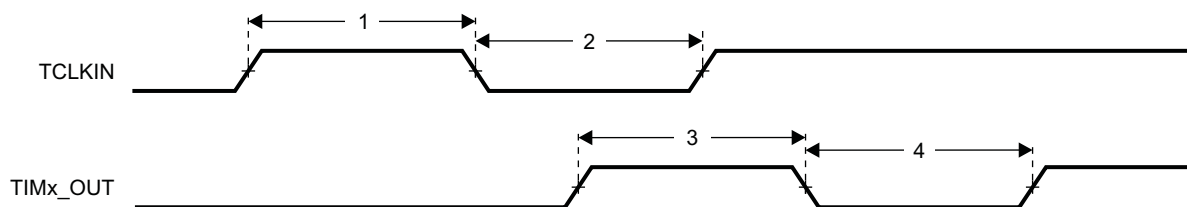
Figure 8-88. Timer Timing
