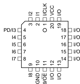
PLCC
