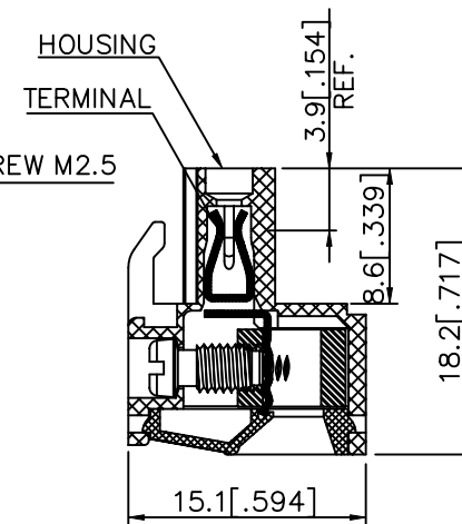
SECTION P-P
