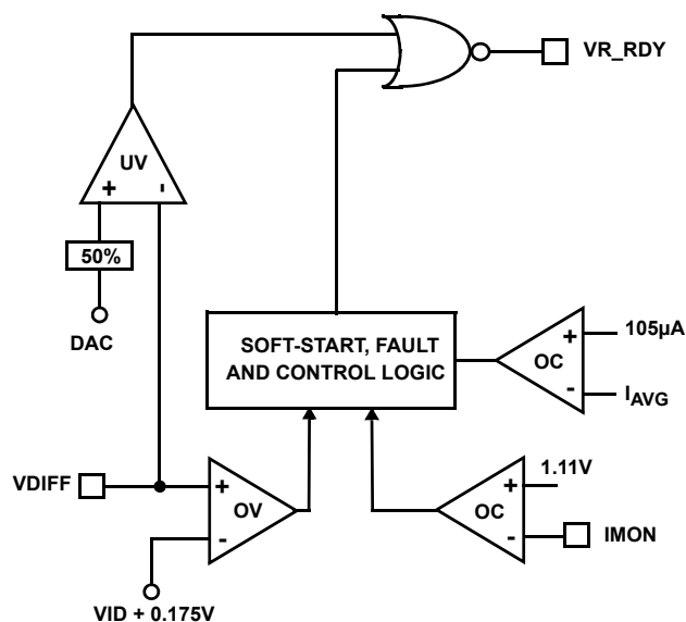
FIGURE 14. VR_RDY AND PROTECTION CIRCUITRY
