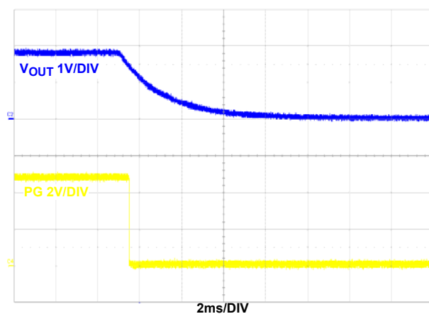
FIGURE 52. OVER-TEMPERATURE PROTECTION
