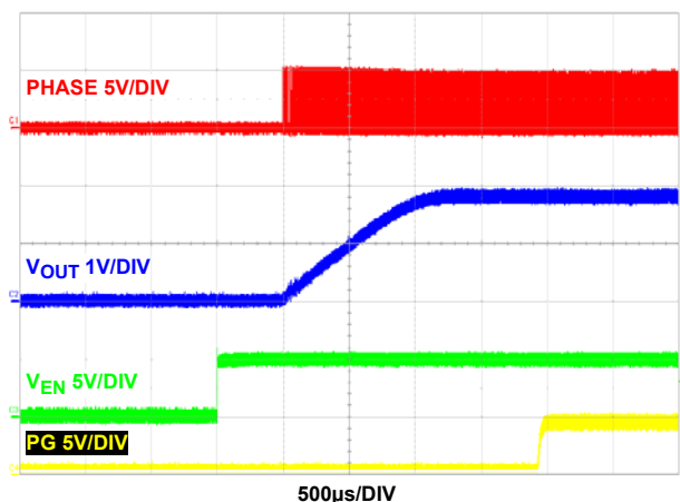
FIGURE 23. START-UP AT 6A LOAD (PWM)
