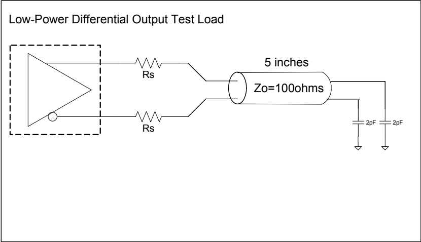
Alternate Differential Output Terminations
