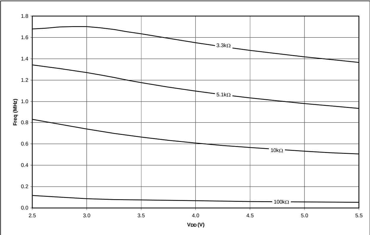
FIGURE 22-11: AVERAGE F_{osc} vs. V_{DD} FOR VARIOUS VALUES OF R (RC MODE, C = 100\text{ pF} , 25^{\circ}\text{C} )
