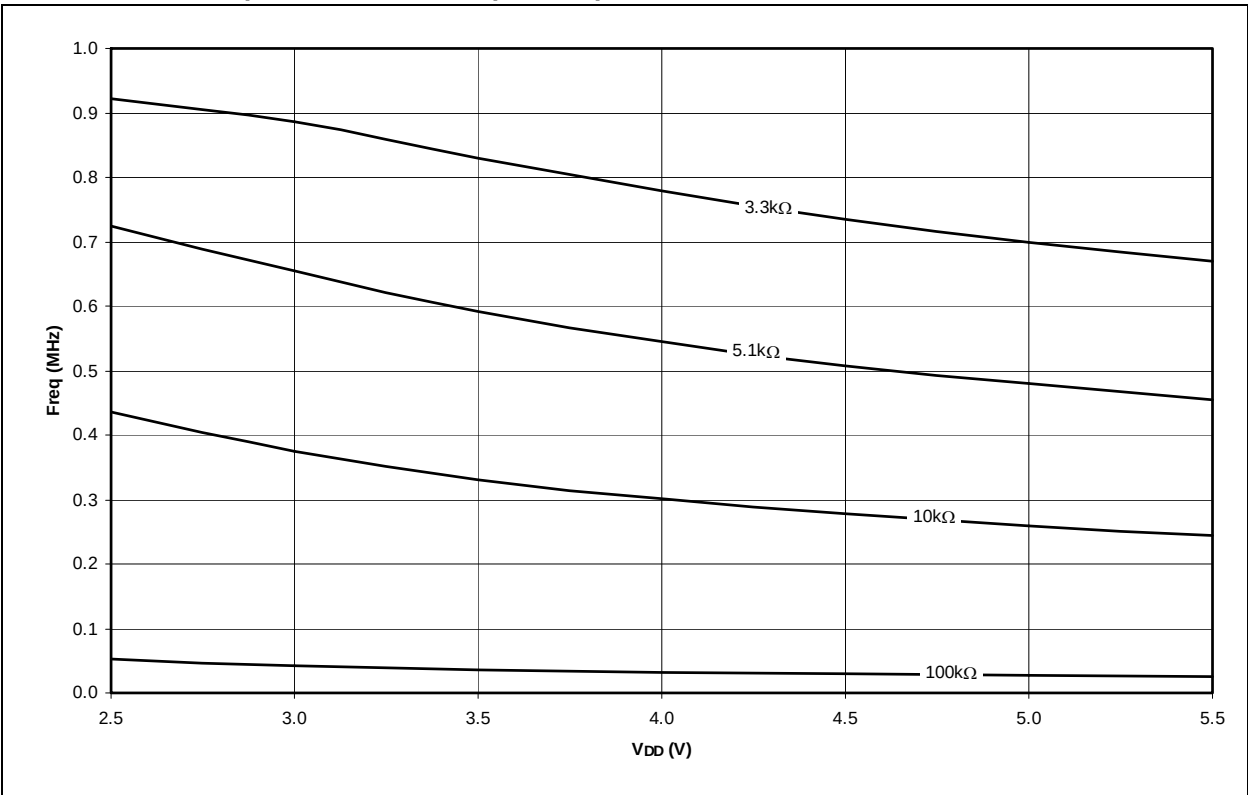
FIGURE 22-12: AVERAGE F_{osc} vs. V_{DD} FOR VARIOUS VALUES OF R (RC MODE, C = 300\text{ pF} , 25^{\circ}\text{C} )
