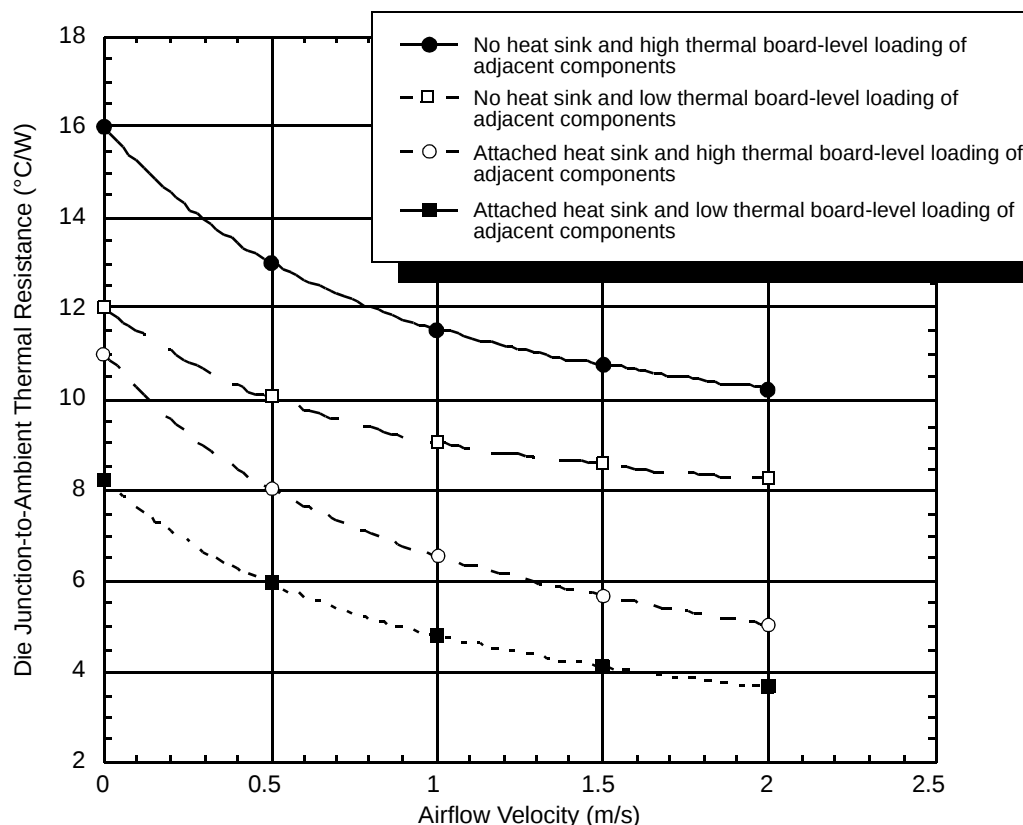
Figure 27. Die Junction-to-Ambient Resistance
